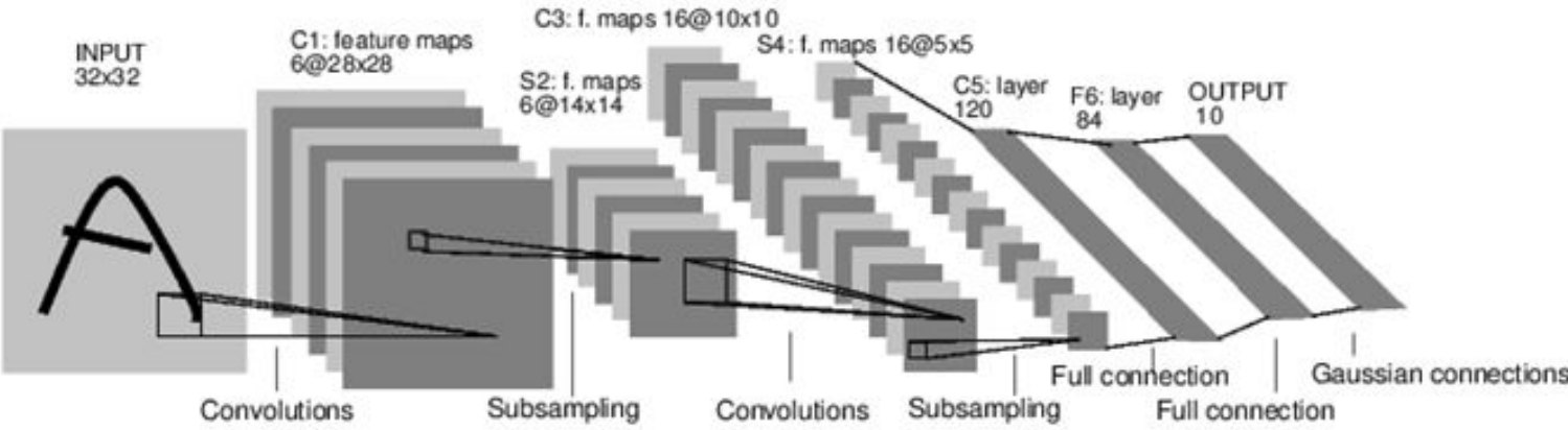
A Full Convolutional Neural Network (LeNet)
